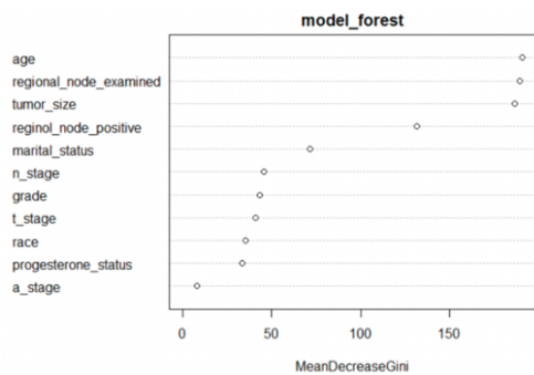
Figure 5 Feature importance for Random Forest. According to the picture, the first 5 most important variables with a mean decreased gini over 50 were selected.
