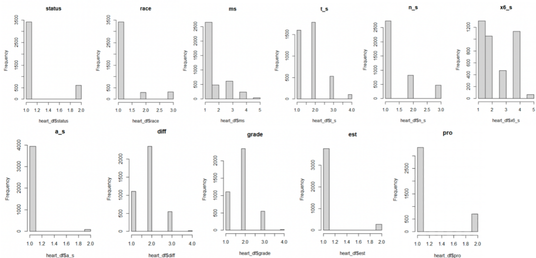
Figure 2 Histogram plots for categorical variables.
