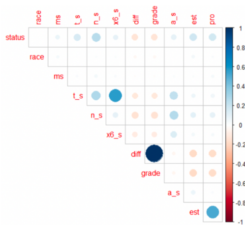
Figure 4 Correlation plots for categorical variables.
