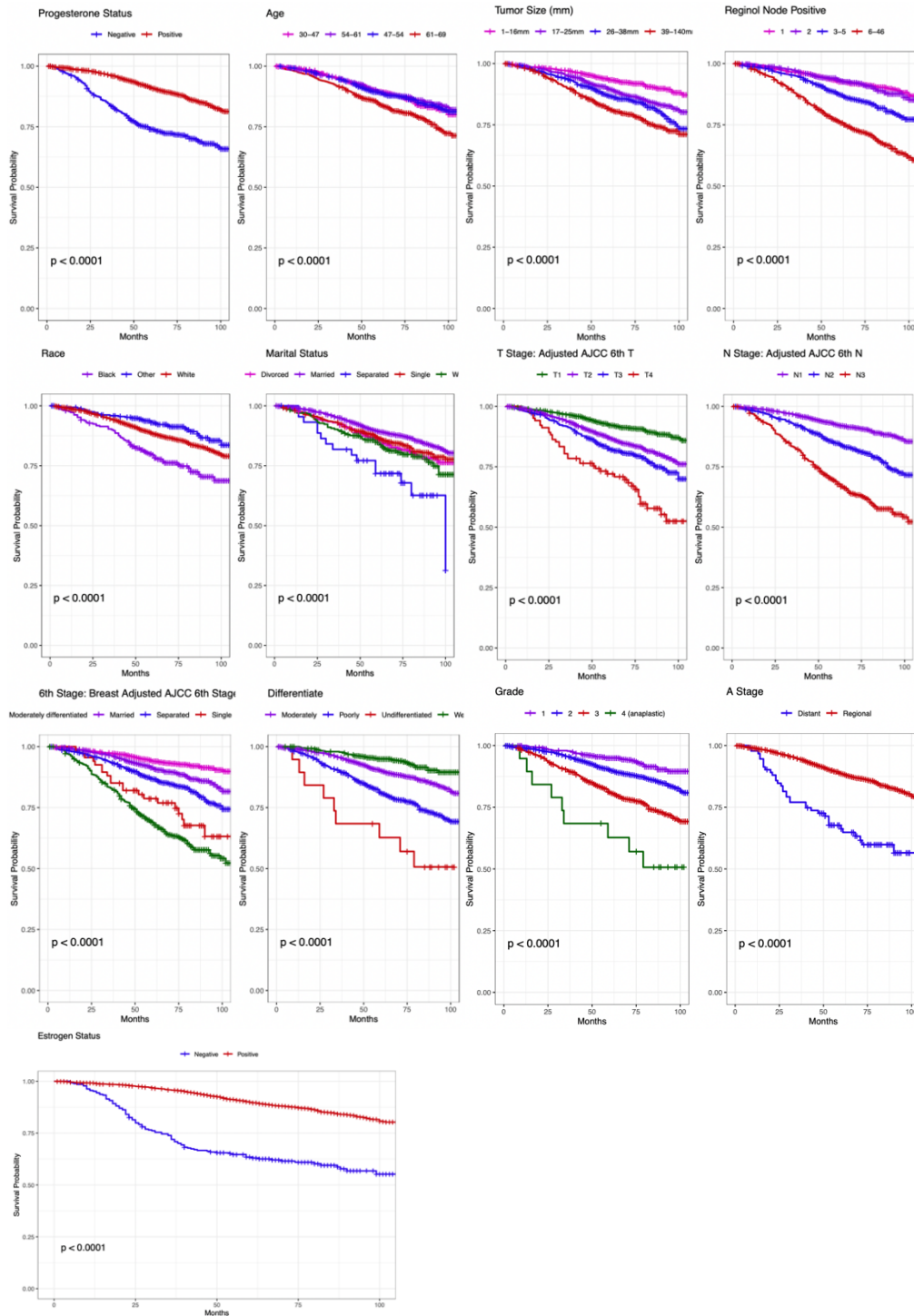
Figure 6 Kaplan-Meier survival curves of variables with a significant log-rank test result. Progesterone status and age exhibit significant differences in survival time, with positive progesterone and the age group 61-69 standing out. Tumor size, regional_node_positivity, race (particularly for Black individuals), marital status (especially for the separated group), t-stage, n-stage (particularly N3), 6th-stage (for widows), differentiate (for undifferentiated individuals), grade (4th level), and distant a-stage display notable variations in survival probabilities. The Estrogen status group also demonstrates significant differences, particularly for negative Estrogen Status.
