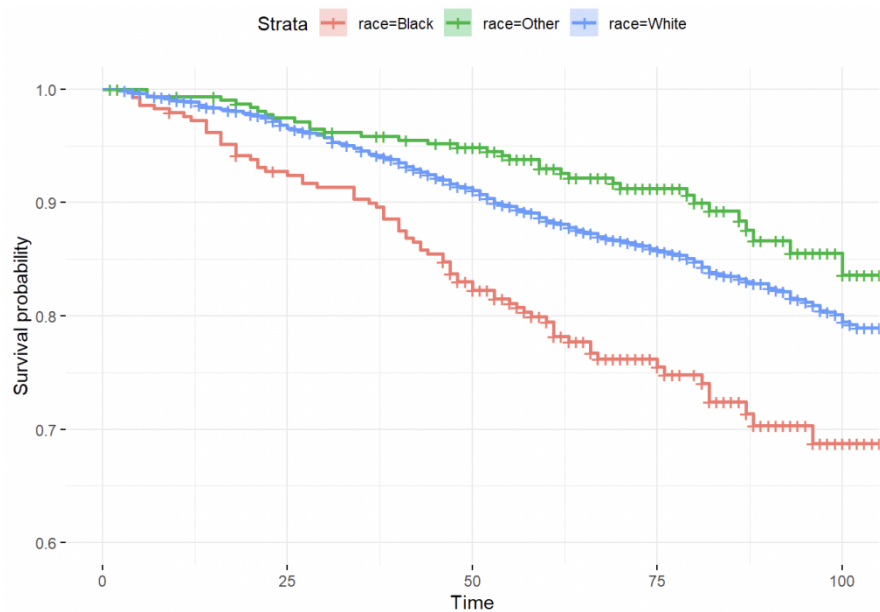
Figure 8 Survival time - survival probability stratified by races.
