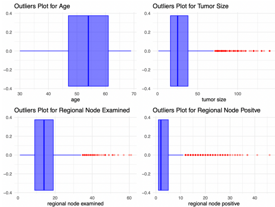
Figure 3 Boxplots for continuous variables to identify outliers.
