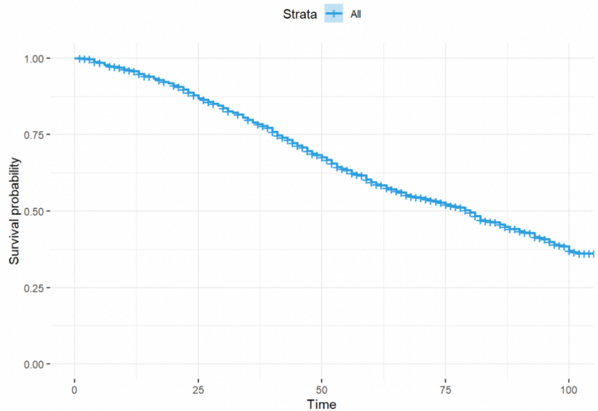
Figure 7 Survival time - survival probability plot by Cox-PH method.
