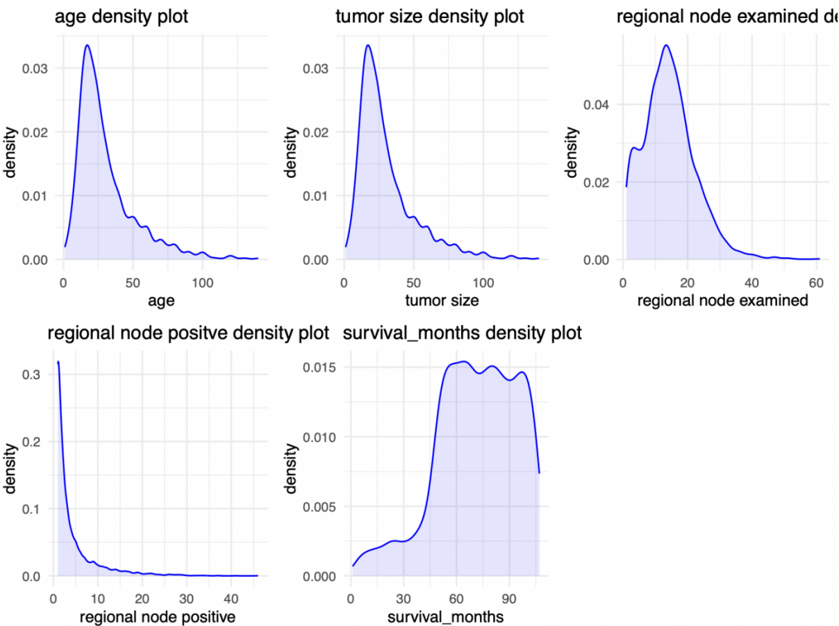
Figure 1 Density plots for all numeric variable
